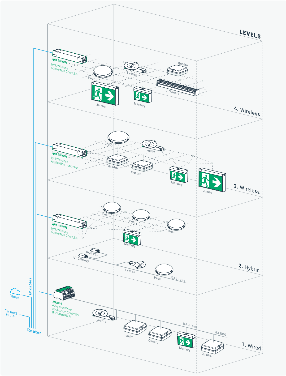
System diagram of multiple Lynk Gateway lines
